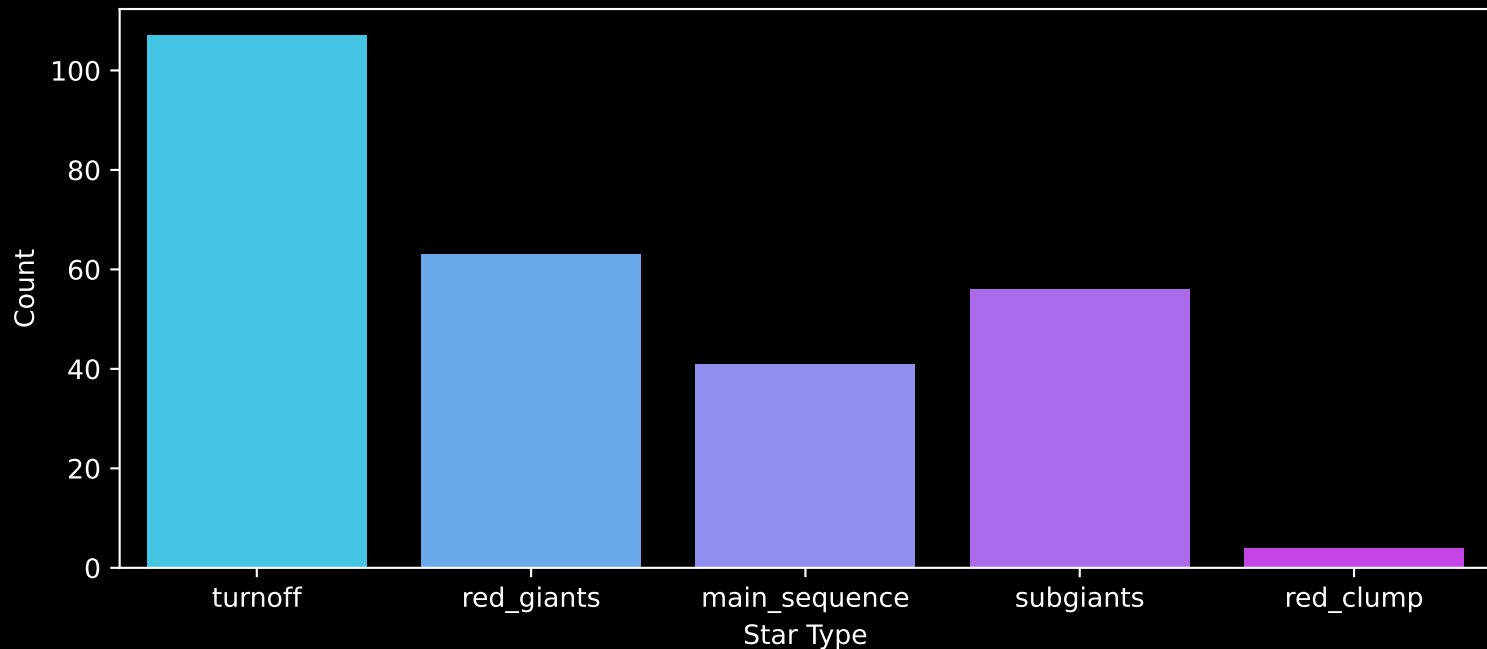
GALAH DR4 Field: [8618] Count plot of Star Type
