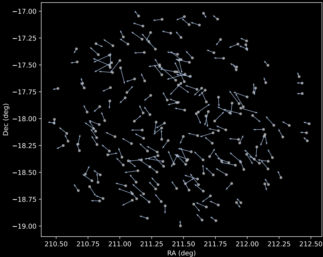
GALAH DR4 Cluster 1 Proper Motion Vectors (n=213)
