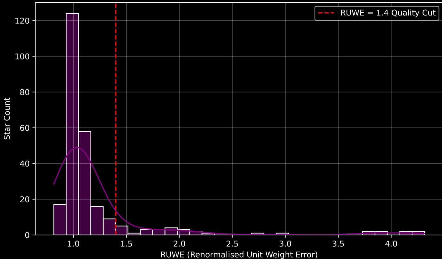
GALAH DR4 Field [8618] RUWE Distribution (n= 256)
